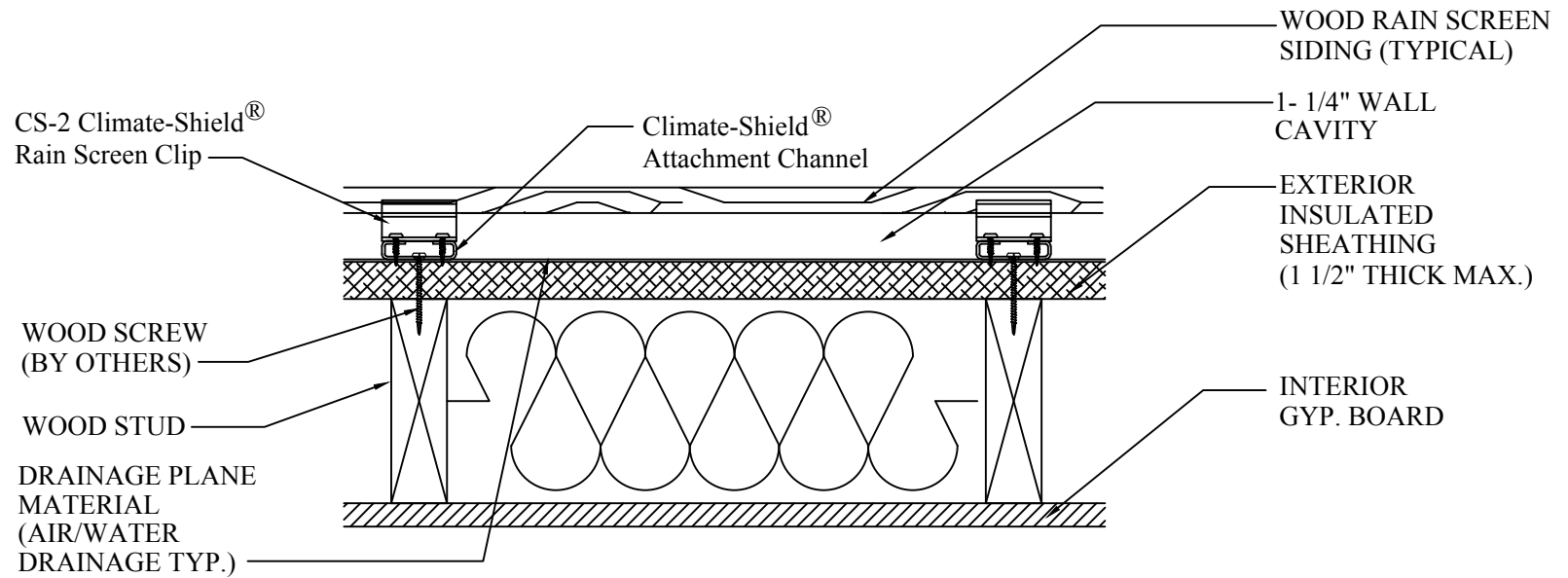
Typ. Exterior Wall System, Plan View
