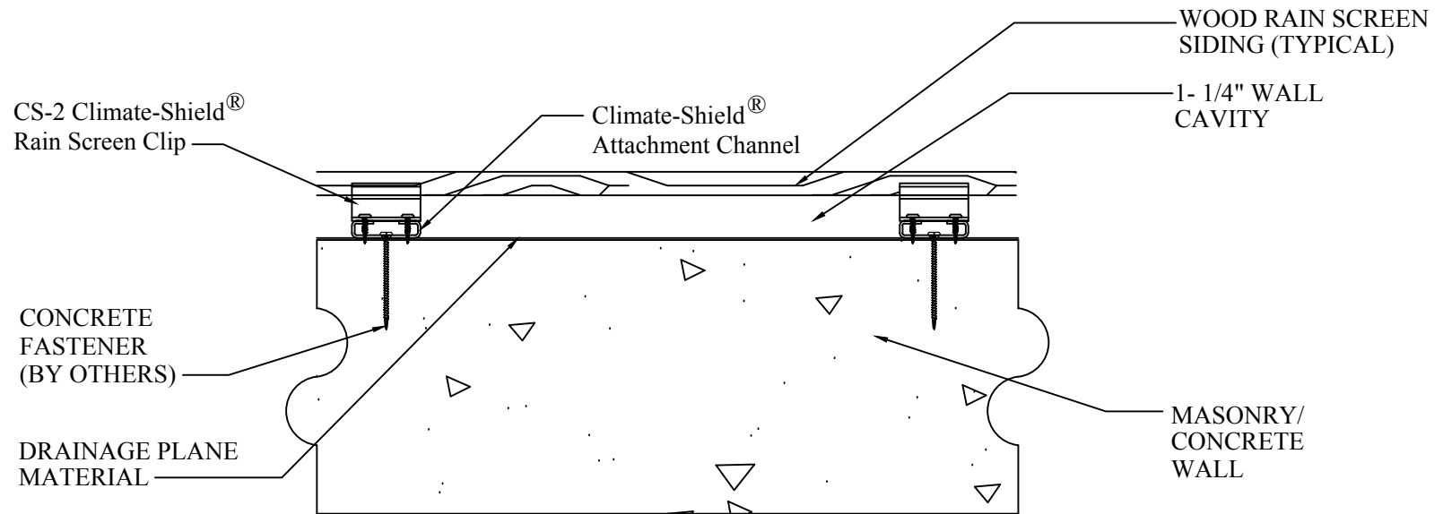
Typ. Concrete Wall System, Plan View
